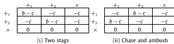
Fig. 2. Examples for m = 2, b > c > 0 . For each combination of contribution ( +_1, +_2 ) and non-contribution ( \times ), entries give fitnesses for the row player.
