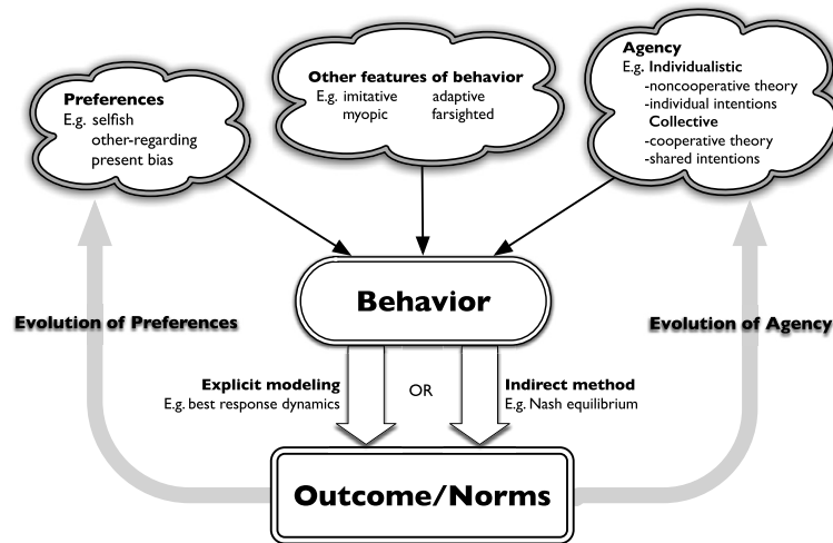
Fig. 1. Behavior embodies aspects of preferences and agency. The interaction of different behaviors leads to outcomes and norms. These in turn determine the type of behavior that is successful and is selected for in the population. Aspects of behavior subject to evolutionary selection include preferences and agency. The current paper studies the evolution of agency.
